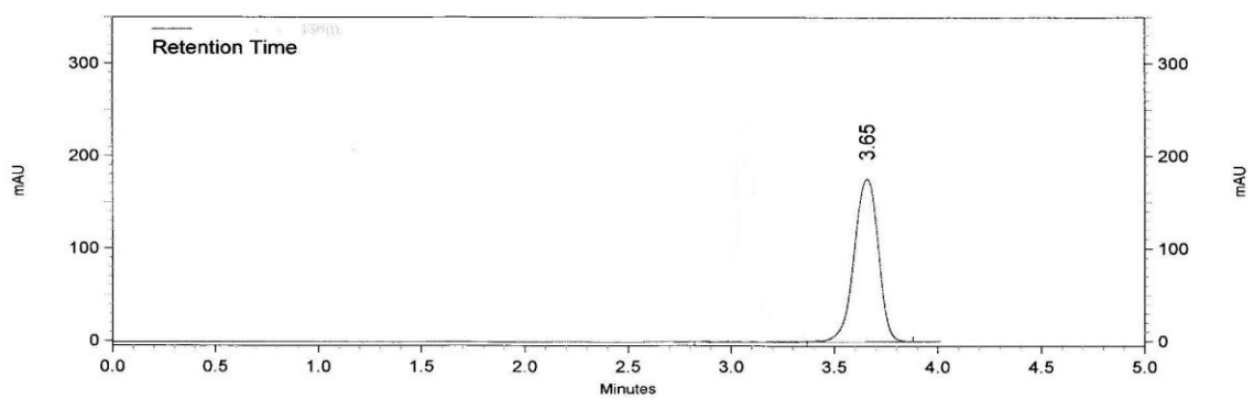
Figure 36: Chromatogram of Sample at normal condition of tadalafil
